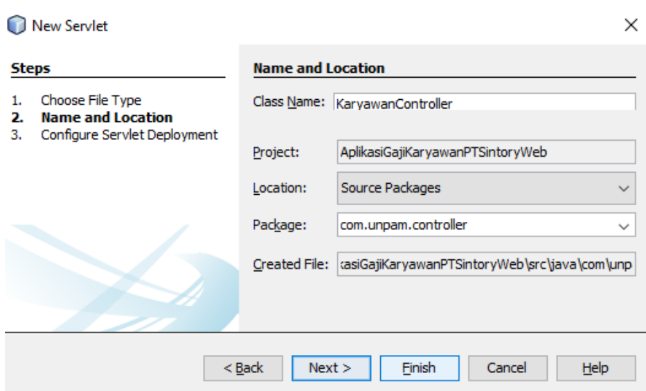
Gambar 245. Class Name
